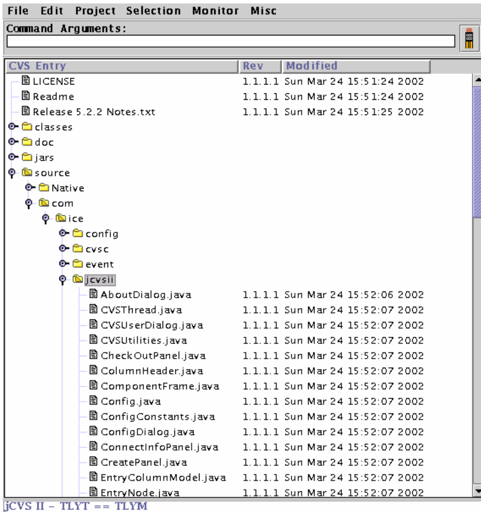
Figure 6-3 The Project Window.
