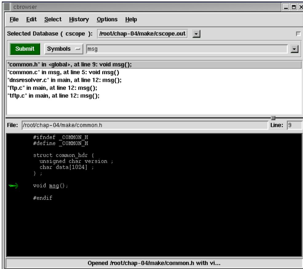
Figure 7-3 The cbrowser window.
