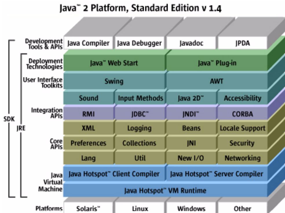
Figure 9-1 Building blocks of J2SE version 1.4.
