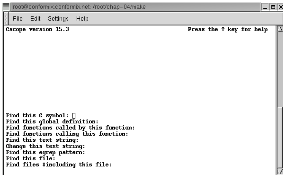
Figure 7-1 The cscope initial screen.
