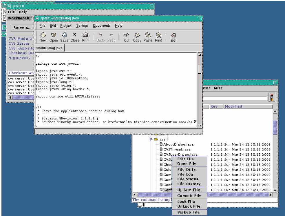
Figure 6-5 Editing source code.
